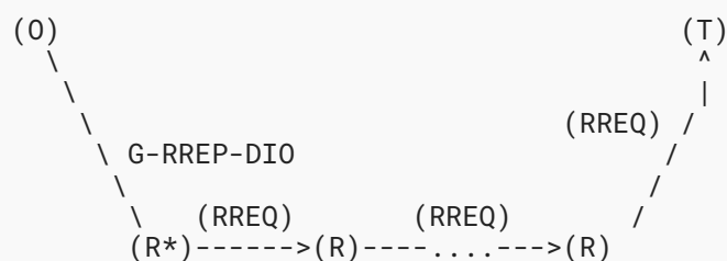
Figure 15: Intermediate Node Initiates G-RREP
